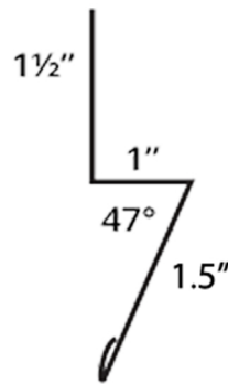
Wall Base
