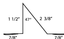
Snow Fence
