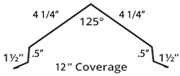
Ridge Cap
