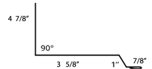
Side Wall
